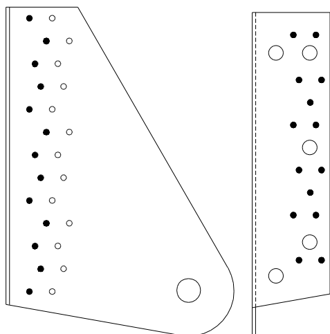
Timber width: b \geq 58 13+14 CNA4,0xl connector nails in face and edge flap of connector
