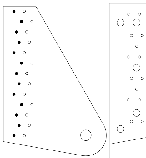
Timber width: b \geq 58 13 CNA4,0xl connector nails in face of connector
