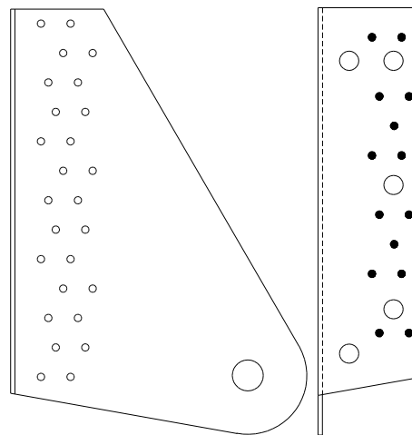
Timber width: b \geq 45 14 CNA4,0xl connector nails in edge flap of connector
