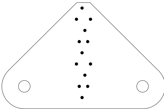
Timber width: b \geq 79 13 CNA4,0xl connector nails in all rows
