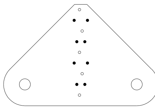
Timber width: b \geq 79 8 CNA4,0xl connector nails in outer rows
