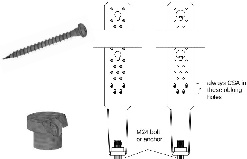
HTT31
